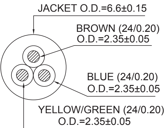
CROSS-SECTION VIEW
