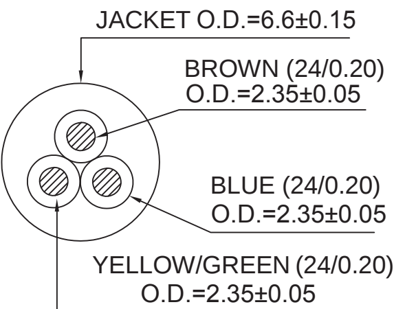
CROSS-SECTION VIEW
