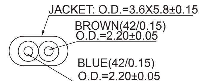
CROSS-SECTION VIEW
