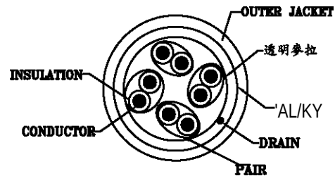
WIRE SECTION
