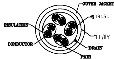
WIRE SECTION
