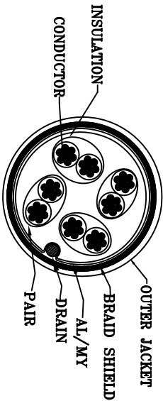
WIRE SECTION
