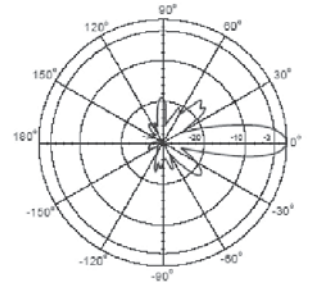
H-plane Co-polarization Pattern (linear, vertical)
