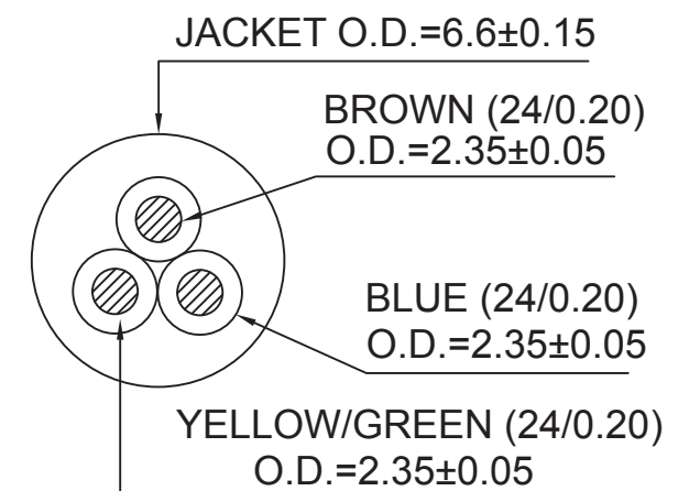
CROSS-SECTION VIEW
