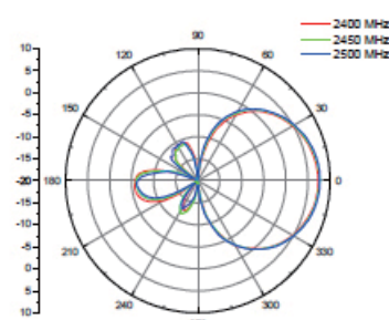
V-plane Co-polarization Pattern
